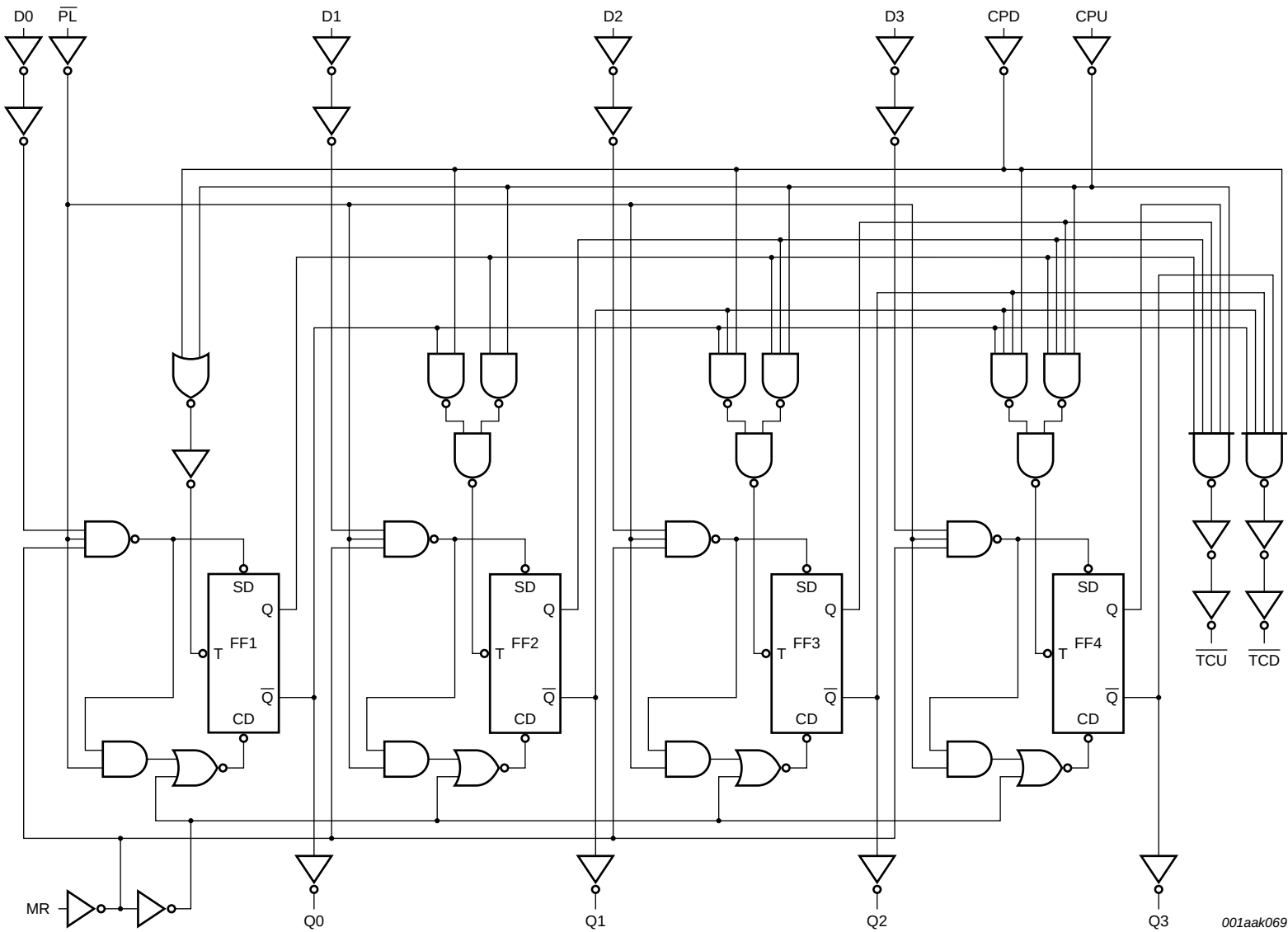
Fig 2. Logic diagram
